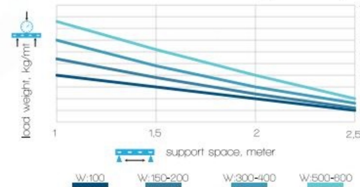
H: 35 - T:4mm Wire Mesh Cable Tray Load Graph
