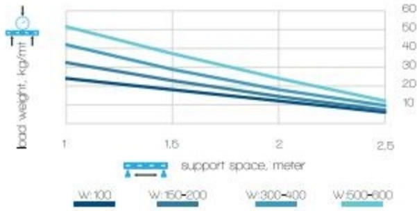
H: 35 - T:4,5mm Wire Mesh Cable Tray Load Graph
