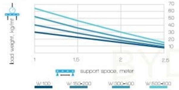
H: 35 - T:5mm Wire Mesh Cable Tray Load Graph
