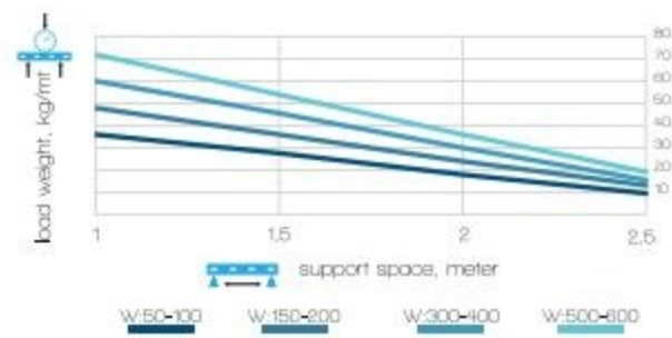
H: 60 - T:4,5mm Wire Mesh Cable Tray Load Graph
