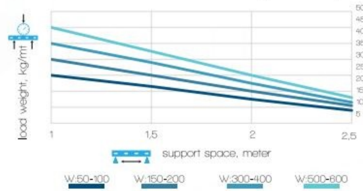
H: 60 - T:4mm Wire Mesh Cable Tray Load Graph
