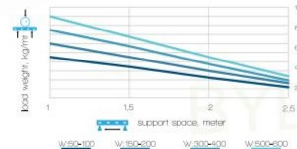
H: 60 - T:5mm Wire Mesh Cable Tray Load Graph
